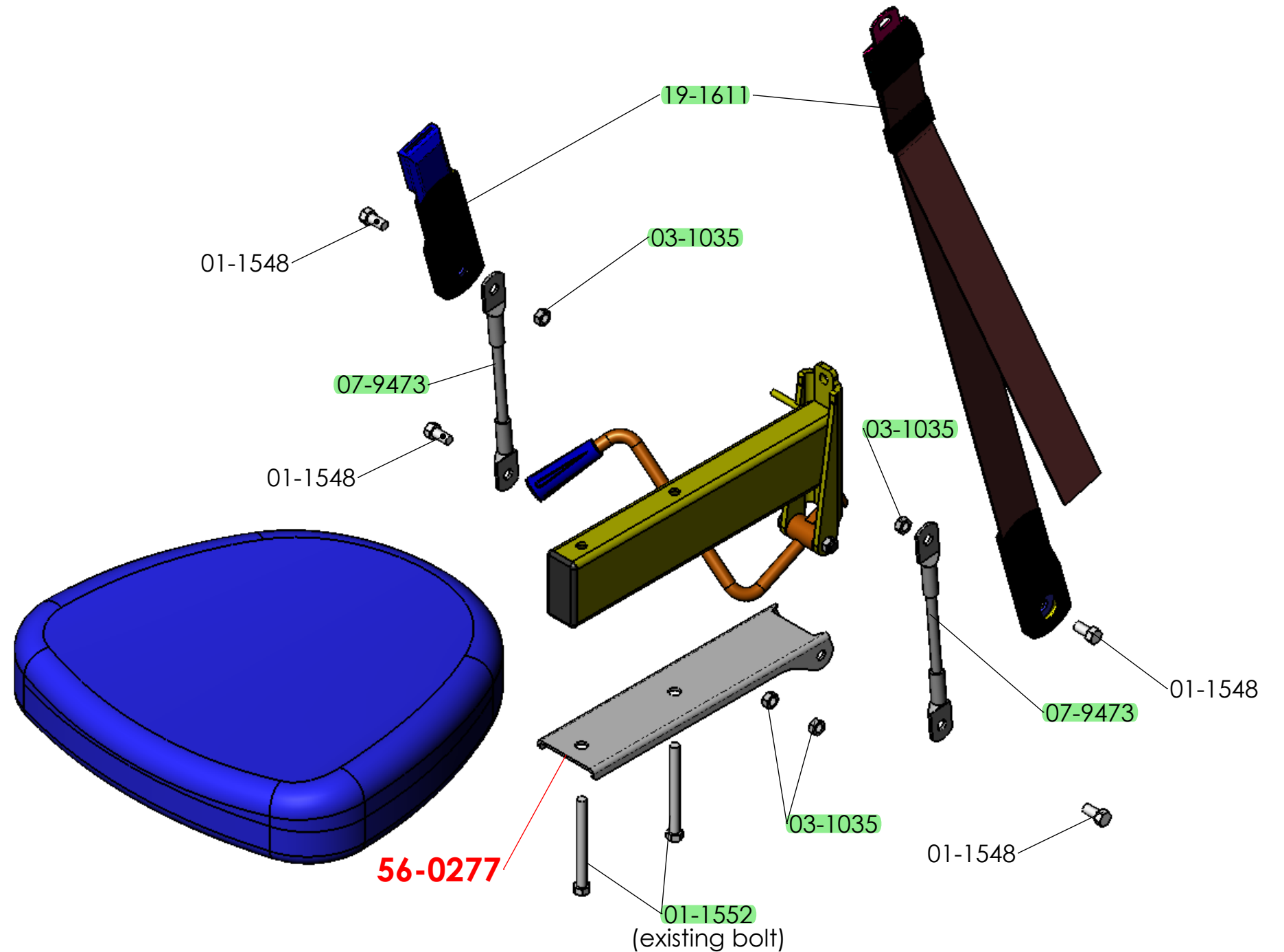
KIT-S6-SB-01 (ONE) S6ABC, LR, VC, OP, BC, TE, PF SEAT BELT ATTACHMENT KIT Parts Diagram
